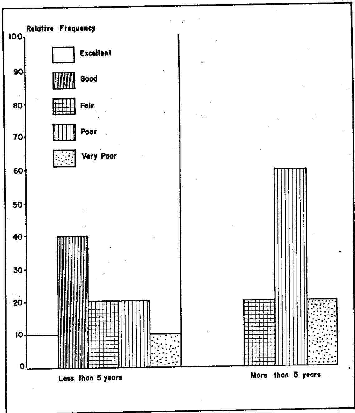
Fig. III.7 - Pasture quality versus occupation time diagrama.
