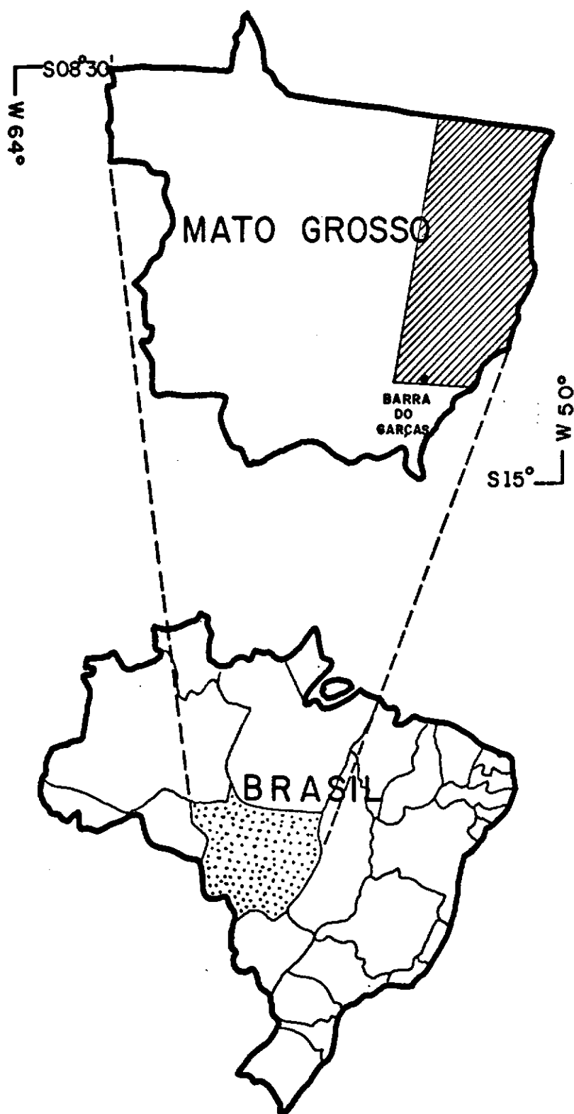
Fig. III.3 - Location map of the study region.
