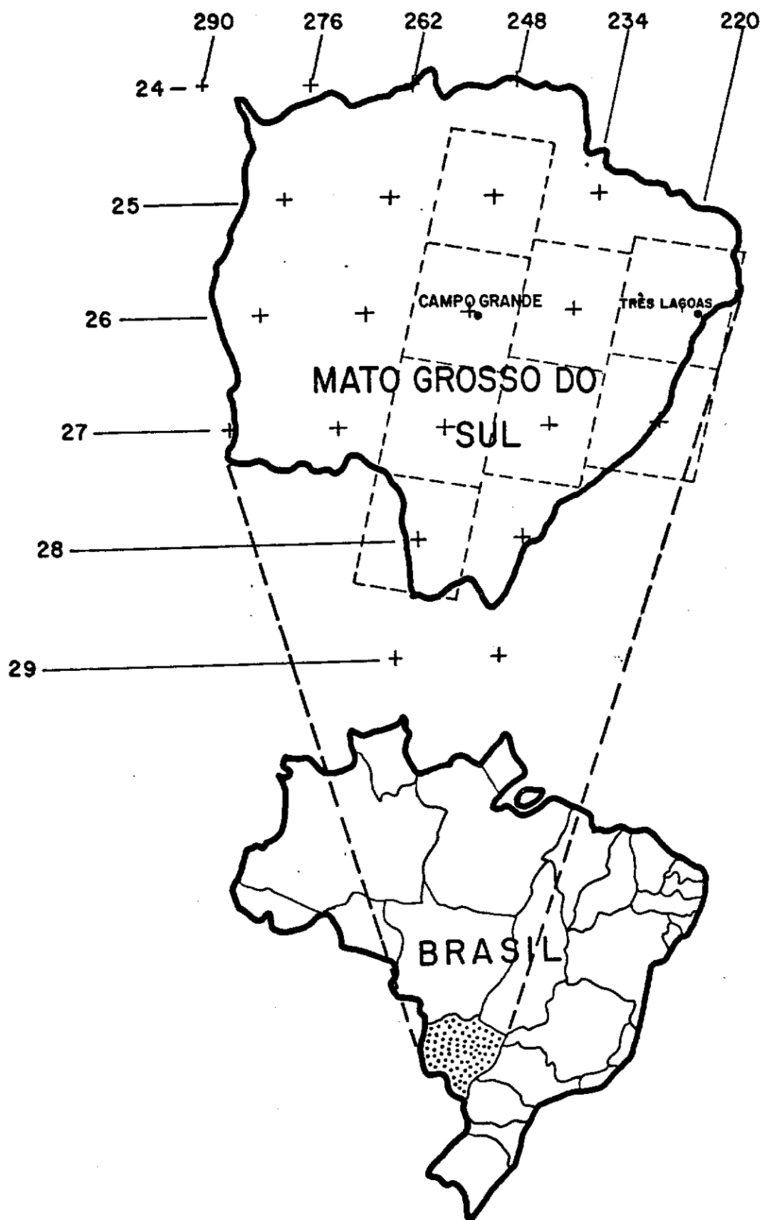
Fig. II.8 - Location map of the study region.
