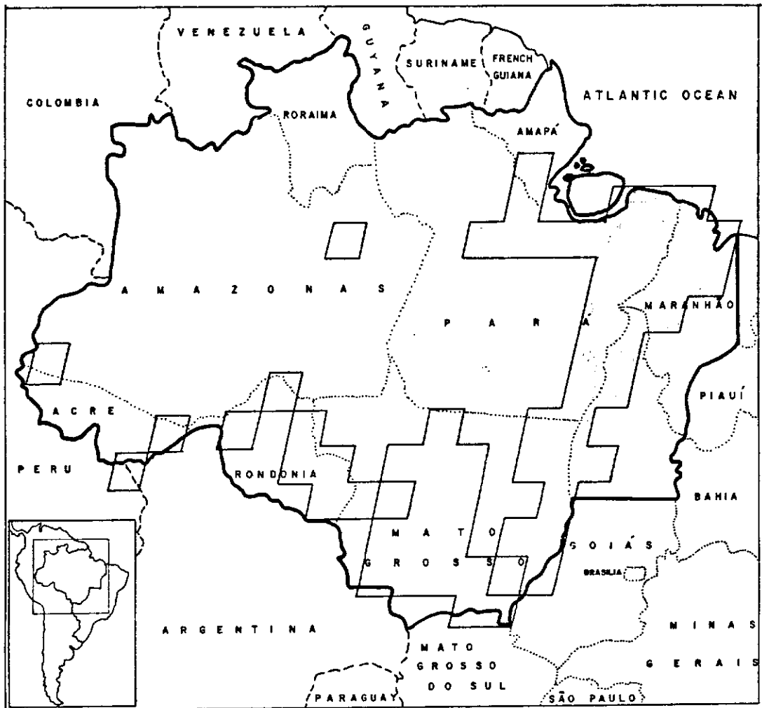
Fig. III.4 - Location map of legal Amazon showing the concentrated deforestation areas.
