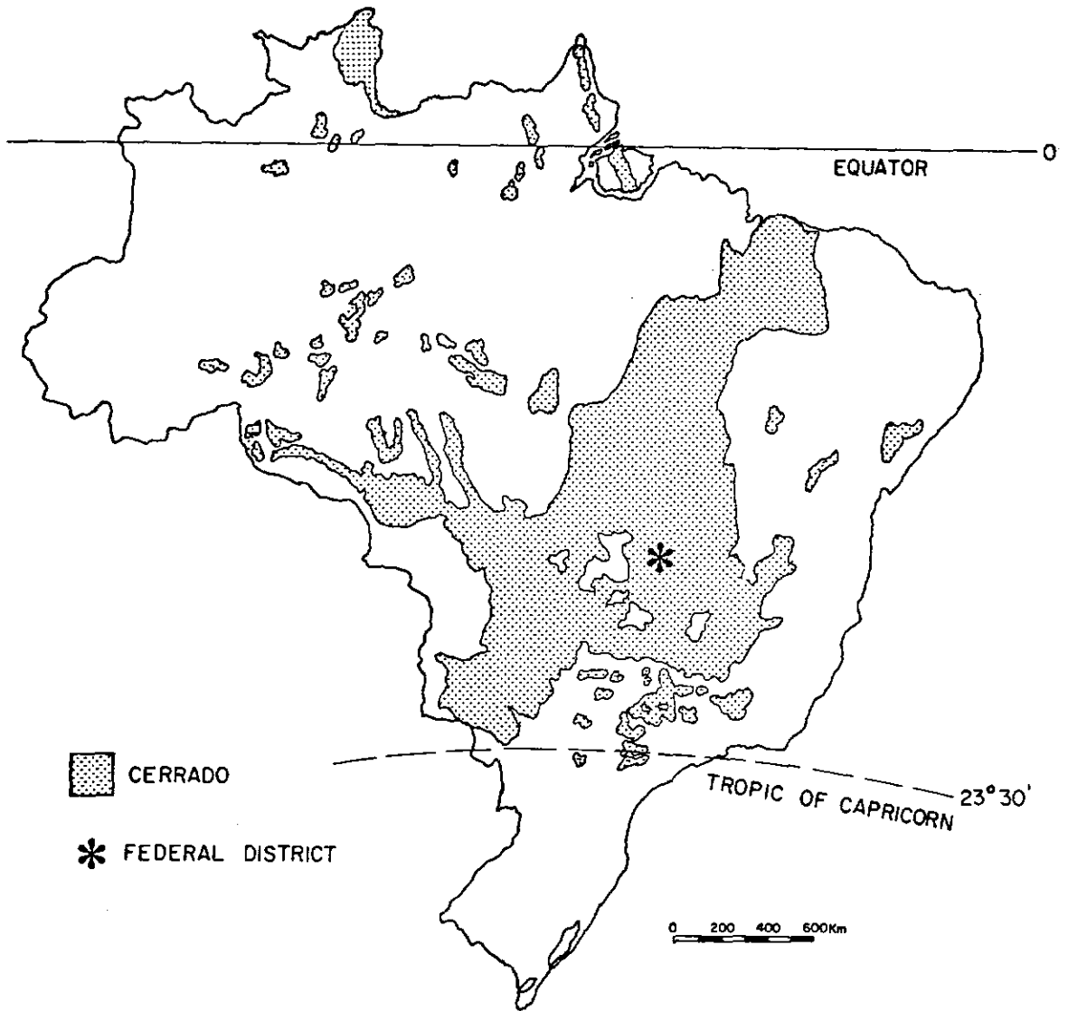
Fig. II.4 - Location of the study area.
