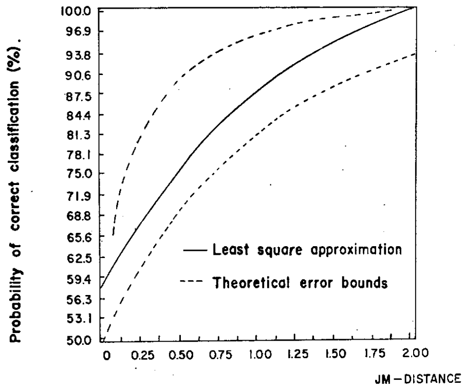
Fig. II.5 - Graph of probability of correct classification of JM distances.
