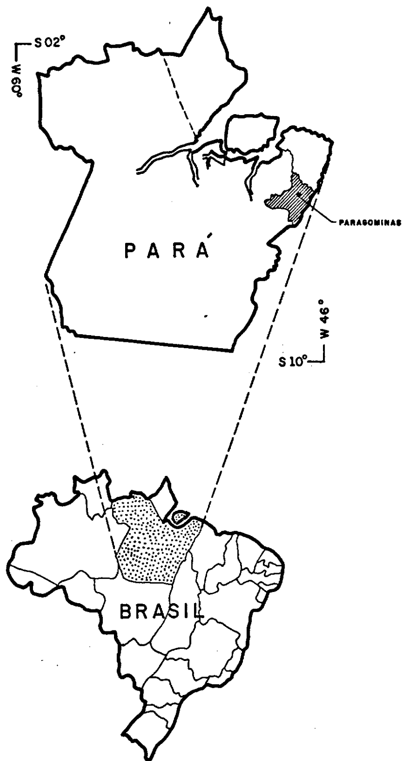
Fig. III.5 - Paragominas Municipality in the Para State.
