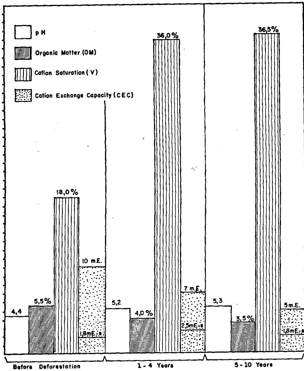
Fig. III.6 - Soil samples analysis.
