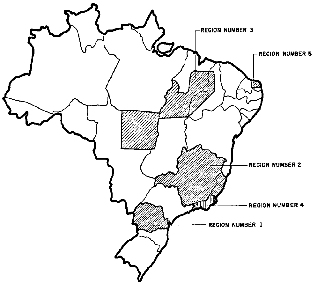
Fig. II.3 - Natural Vegetation Applications study Areas.
