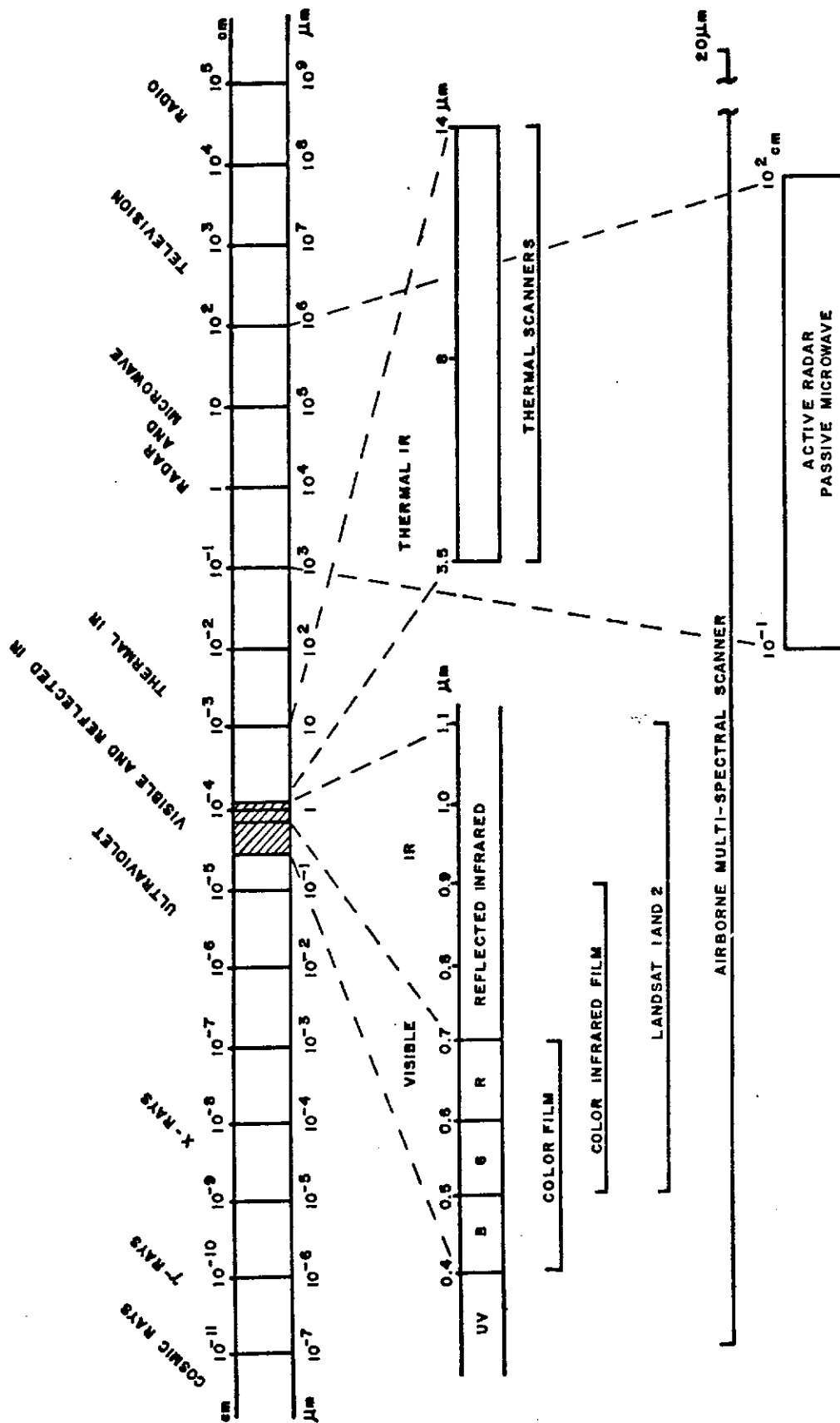
Fig. II.2 - The Electromagnetic Spectrum with Spectral Ranges of Some Common Remote Sensing Systems. From: Harding and Scott (1978), p. 110
