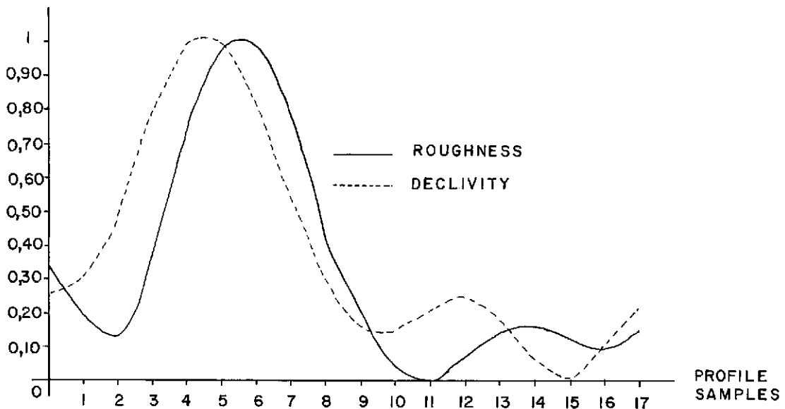
FIGURE III.4 - COMPARISON BETWEEN ROUGHNESS INDEX AND TOPOGRAPHIC TEXTURE, ROUGHNESS INDEX AND DECLIVITY RELATIVE TO THE PROFILES WITH STANDARDIZED VALUES ACQUIRED FROM THE EIGHTH DEGREE TREND SURFACE.
