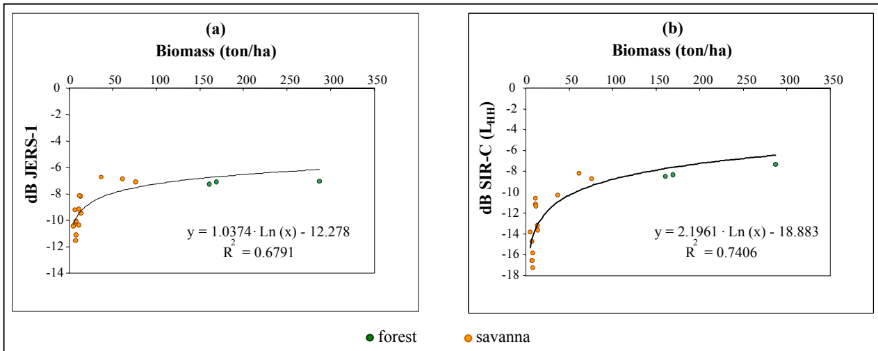
Figure 3. Correlation between biomass and JERS-1 (a) or SIR-C/L HH band (b) backscatter values for forest and savanna formations.
