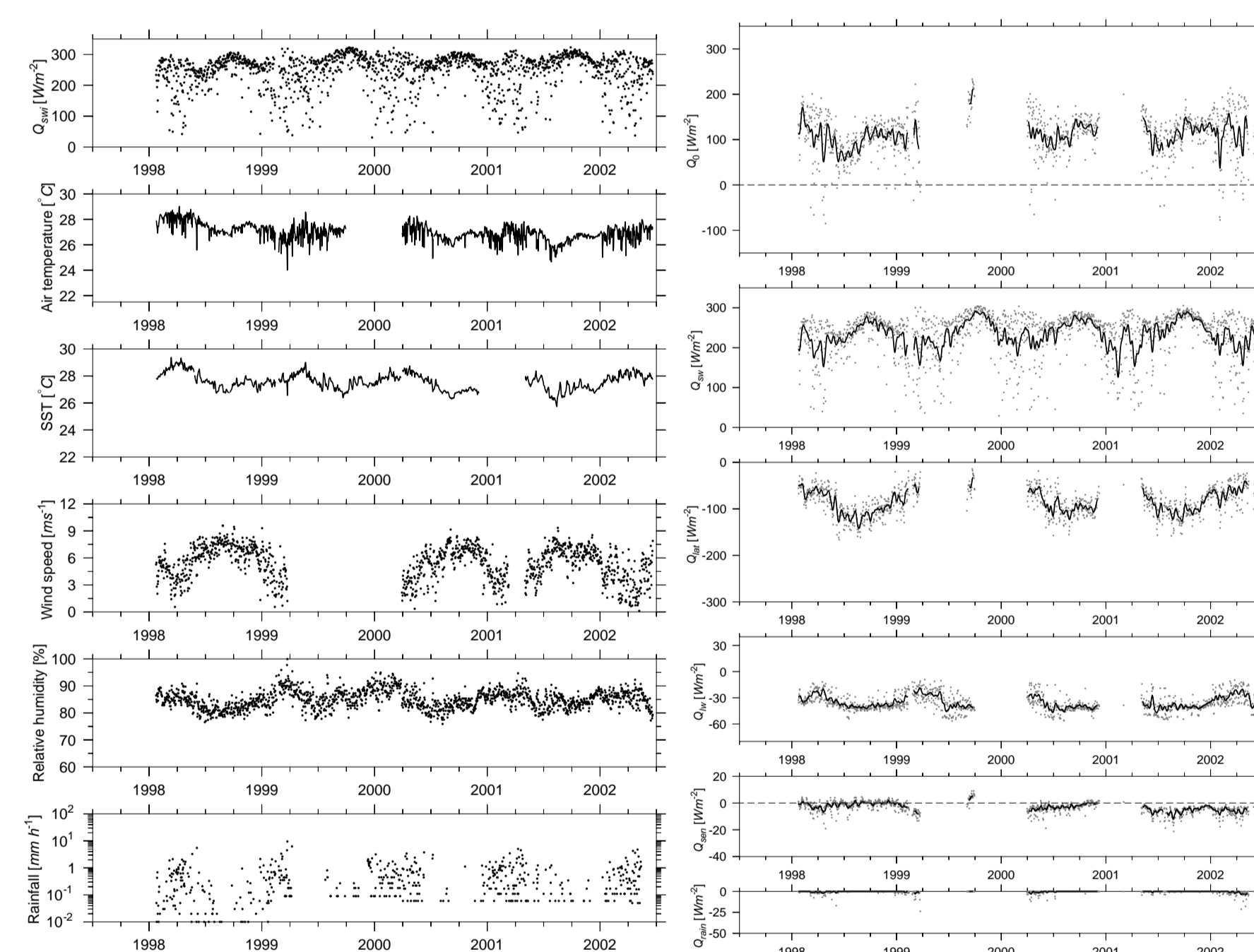
FIGURE 4: Variables measured from buoy 00° 35°W (left) and surface heat flux components.
