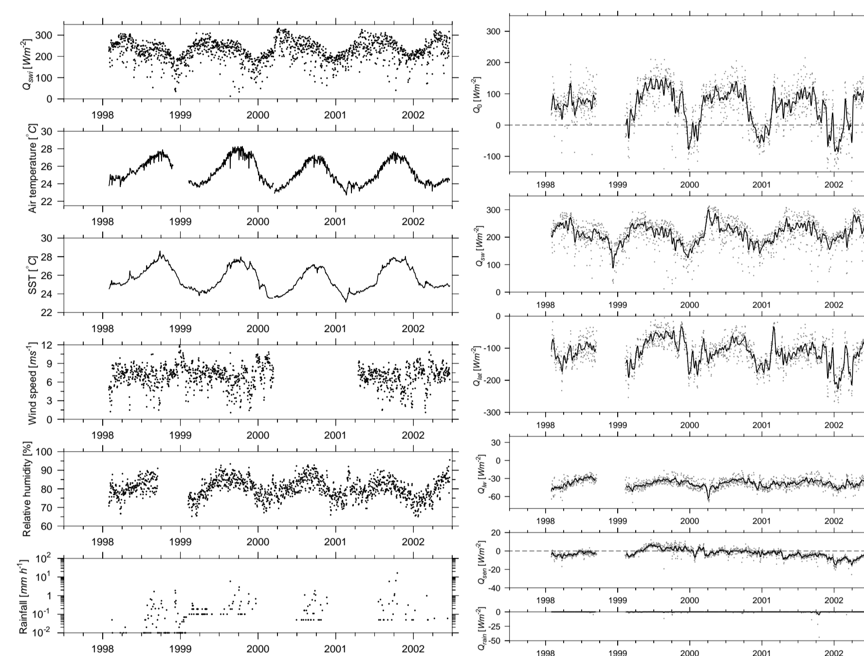
FIGURE 3: Variables measured from buoy 15°N 38°W (left) and surface heat flux components.
