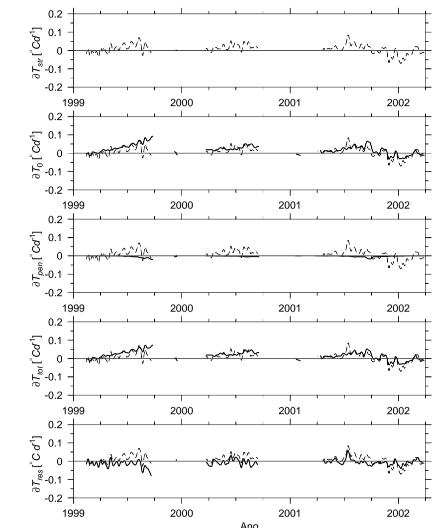
FIGURE 5: Temperature variation tendency by the different heat fluxes
