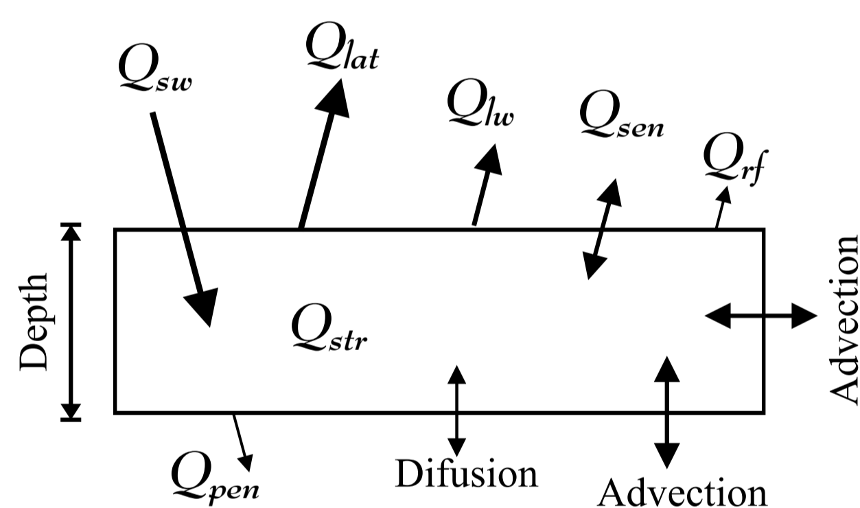
FIGURE 2: Heat fluxes components of mixed layer.
