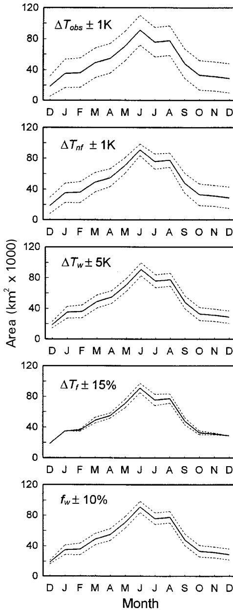
Figure 2. Sensitivity analysis of the algorithm (equation (3)) for estimation of flooded area using data from 1982 as an example. The solid line shows the original flooded area estimates and the dashed lines show the results when a particular input term (as noted on each graph) is varied.
