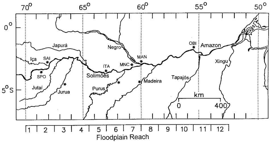
Figure 1. The Amazon River and its major tributaries. Flooded area was estimated for the 12 longitudinal reaches shown along the bottom of the map. Flooded area was also estimated for the Purus, Madeira and Jurua Rivers from 8° S (the southern border of this map) to their confluences with the Amazon River. River stage stations are marked by an asterisk; codes are as follows: SPO, São Paulo de Olivença; SAI, Santo Antônio de Iça; ITA, Itapeua; MNC, Manacapuru; MAN, Manaus; OBI, Obidos. The Jurua River stage station is at Carauari, the Purus River station is at Beruri, and the Madeira River station is at Borba.
