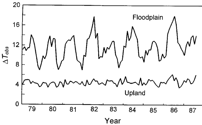
Figure 6. Comparison of the \Delta T_{obs} over the floodplain of the Amazon River main stem (mean for two grid cells in reach 6) with the \Delta T_{obs} over nearby upland areas (mean for five grid cells adjacent to reach 6). These data were selected as an example to show the effect of seasonal inundation on \Delta T_{obs} .
