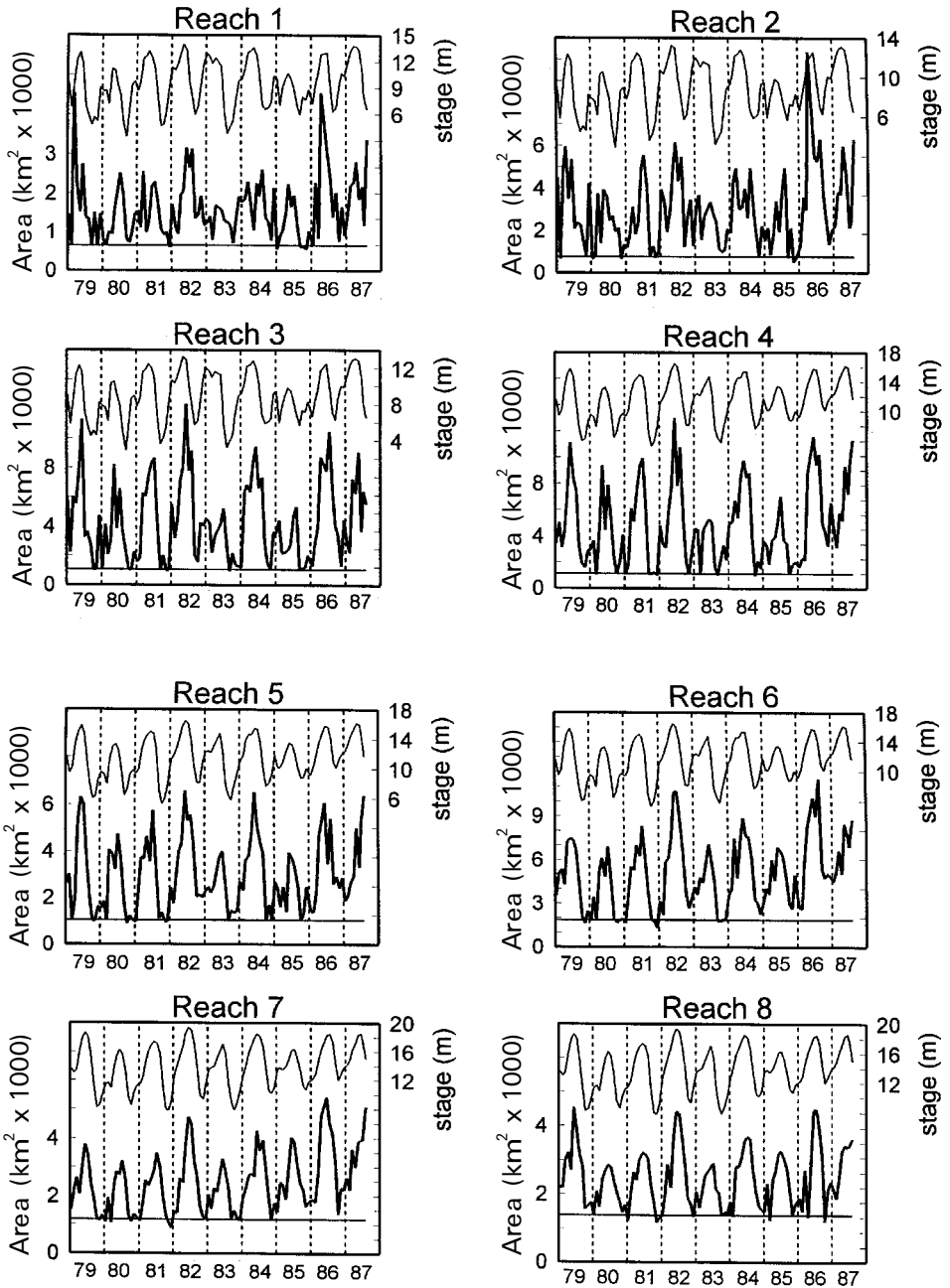
Figure 3. Monthly estimates of the total flooded area (inundated floodplain plus rivers and lakes) for each reach of the Amazon River main stem. Flooded area is depicted by bold lines, with the river stage plotted above for comparison (stage stations corresponding to each reach are identified in table 3). The horizontal lines show the open-water areas from table 1. When the flooded area is at or below the horizontal line, no floodplain is inundated and only open water is present.
