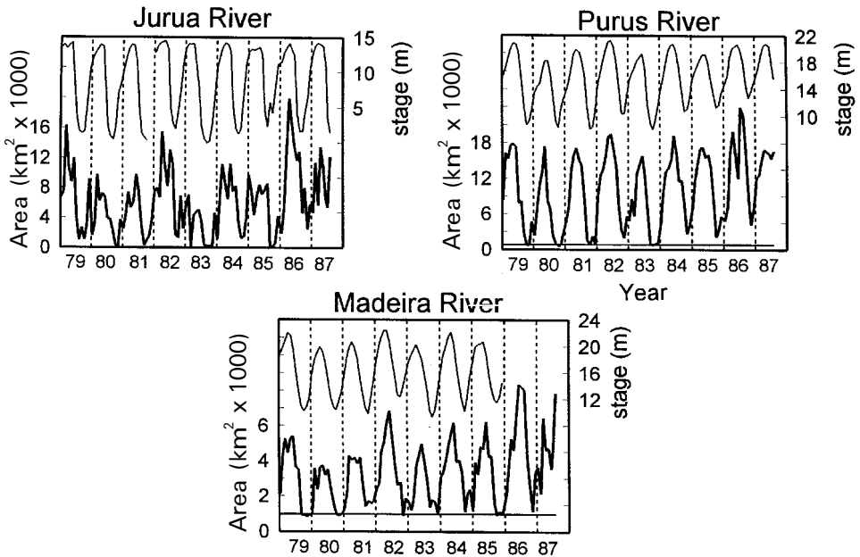
Figure 5. Monthly estimates of total flooded area (inundated floodplain plus rivers and lakes) for the Jurua, Purus and Madeira rivers, three major tributaries of the Amazon River. Flooded area is depicted as bold lines, with the available river stage plotted above for comparison (stage stations are identified in table 3). The horizontal lines show the open-water areas from table 1 (open-water area is insignificant in the Jurua River). When the flooded area is at or below the horizontal line, no floodplain is inundated and only open water is present.
