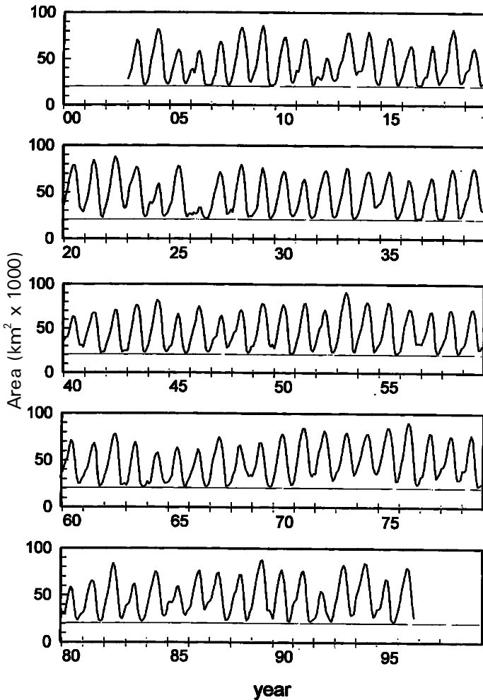
Figure 9. A 94-year reconstruction of flooded area (inundated floodplain plus rivers and lakes) from the river stage record, based on the relationship in figure 8. The horizontal line shows the total open-water area (river channels plus permanent floodplain lakes). The long-term mean of the flooded area along the Amazon River main stem is 46\,830\text{ km}^2 .
