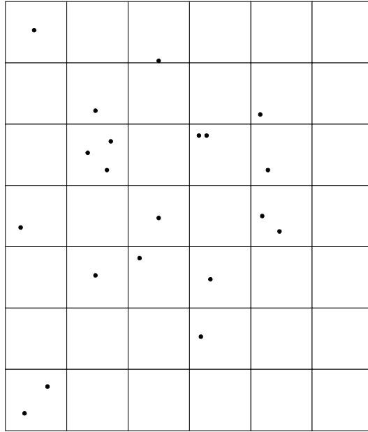
Figura 6.11 – Grid File.
