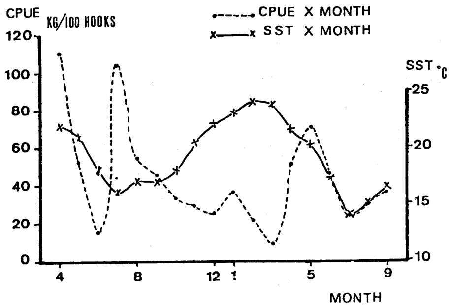
Fig. 5 - Monthly variations of bigeye tuna CPUE and SST for Apr., 1978 - Sept., 1979.
